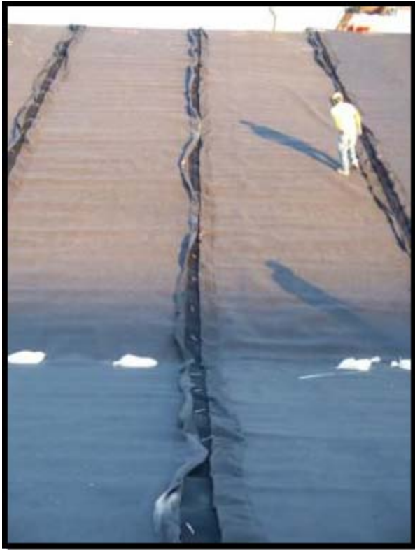
Geocomposite Seaming
