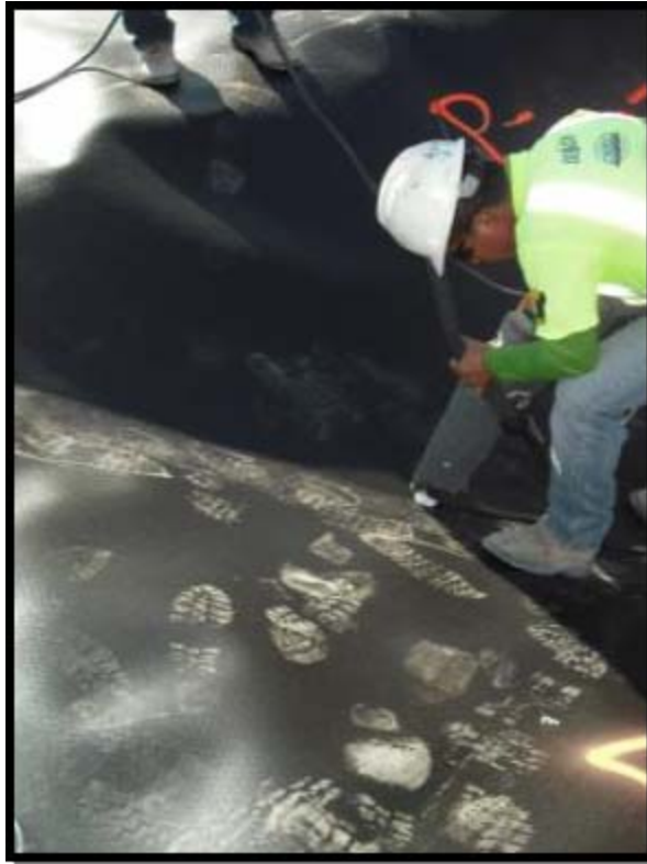
Extrusion Welding
