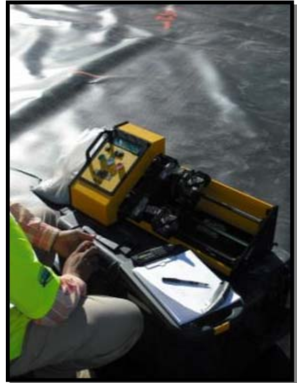
Trial Weld
